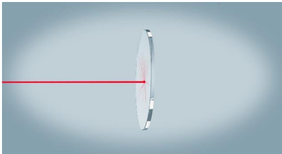
Absorption
