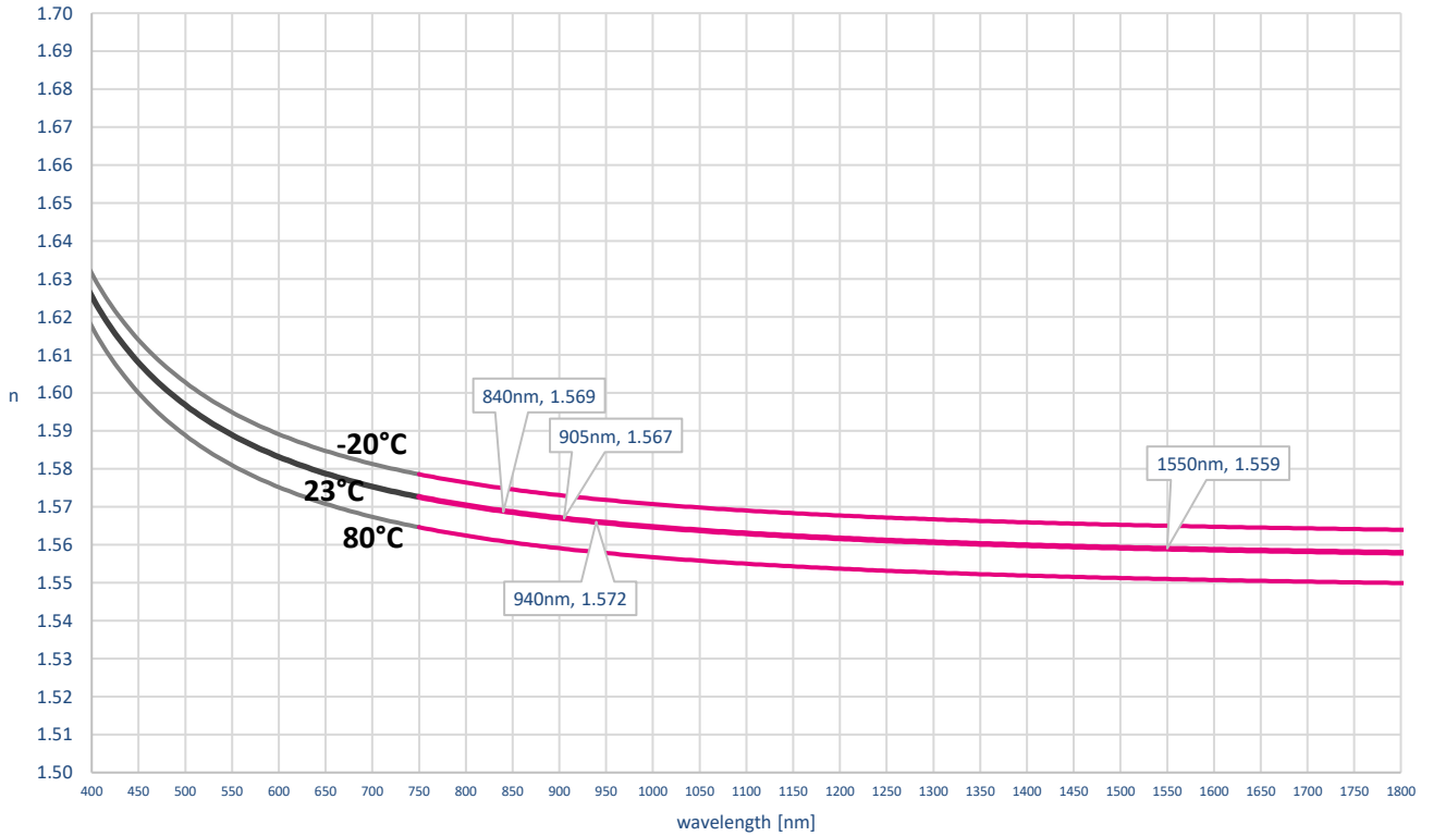
Refractive Index of Makrolon® in the IR range
