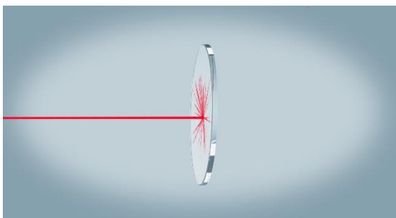
Internal scattering
