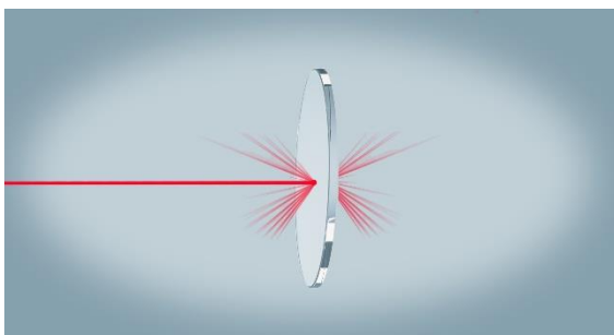
Surface scattering
